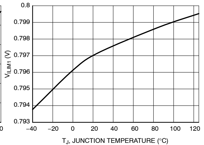
Figure 61. V_{LIM1} vs. Temperature
